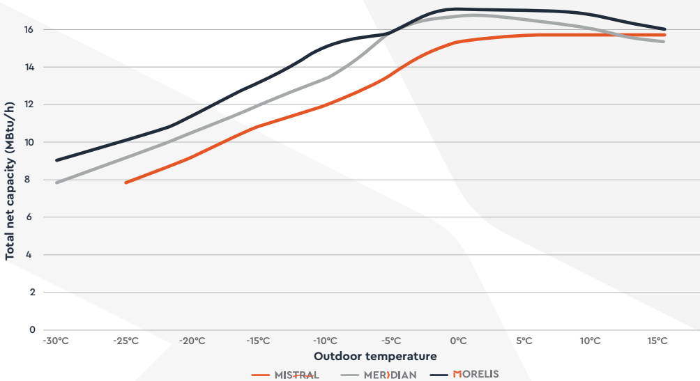
Graphical representation of 12,000 Btu models for an indoor temperature of 21°C
